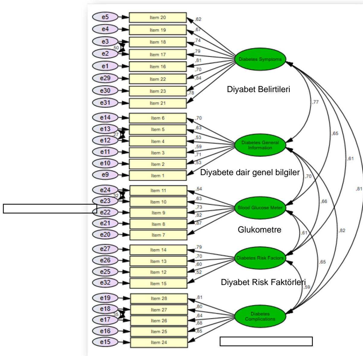
Figure 1. The Diabetes Knowledge Scale for Adults Path Diagram and Standardized Analysis Results
