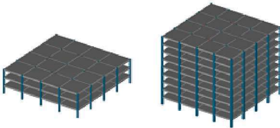
Fig.3. 3D RC structure for 3 and 9-stories
