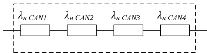
Figure 4 – RLSFB of SAN boards before the reconfiguration of the SAN interface The reconfiguration consists in organizing two channels of the SAN interface for each group of objects not within the framework of one SAN board, but on two ports on different (adjacent) SAN boards according to the principle shown in Figure 5.
