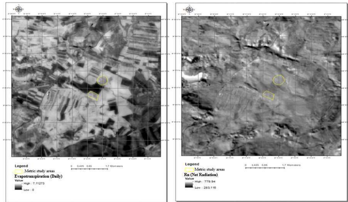
Figure 4. Metric algorithm results on May 2, 2023, raster outputs
