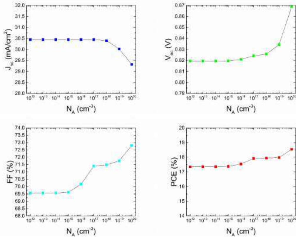
Figure 2. Effect of the acceptor concentration of CdTe as HTL on the performance parameters of the device.
