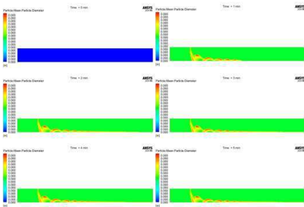
Figure 5. Time-dependent particle distribution of Chemosil 211 material
