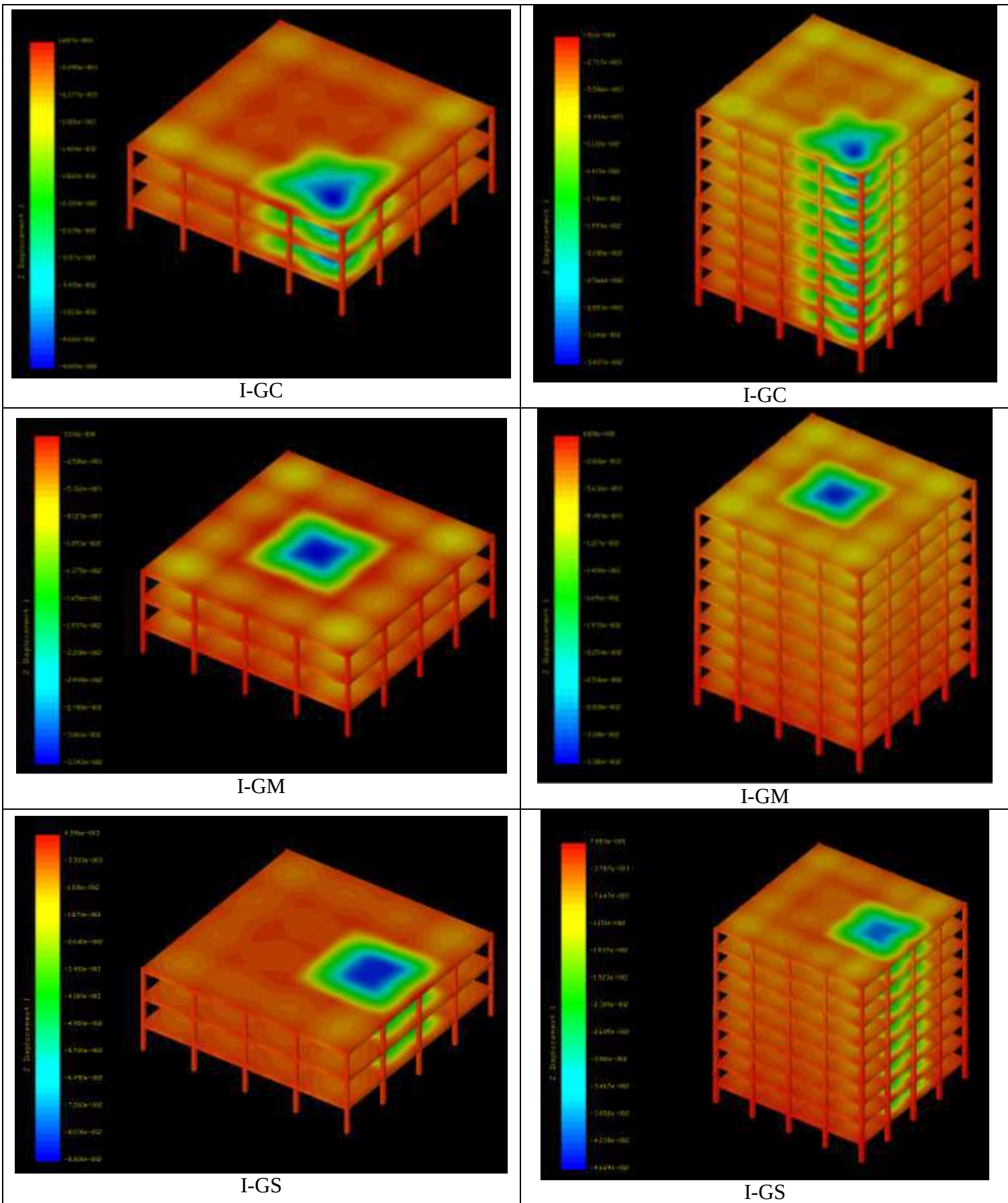
Fig. 5 Vertical displacements for both external and internal column removal scenarios on the ground floor.
