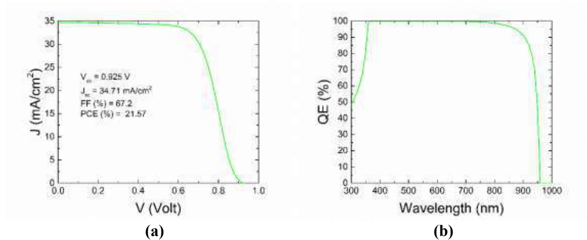
Figure 2. a) The J-V curve and b) the QE curve obtained by simulation for the device. Solar cells are made to function in a variety of temperature environments when used in real time. Because of the greater temperature-induced thermal stresses in the absorber layer, an increase in operating temperature may result in subpar device performance. As such, it is equally critical to analyze the device performance at various operating temperatures. Fig. 3 illustrates how temperature changes affect the device performance parameters. The J_{sc} remains unchanged with temperature. The V_{oc} and FF of the device show a linear decline at only higher temperatures, which only lowers the device performance at higher temperatures. The increase in reverse saturation current with a rise in operating temperature is responsible for the decrease in V_{oc} . The PCE is mainly maintained in the investigated temperature region, confirming that the device is highly stable.
