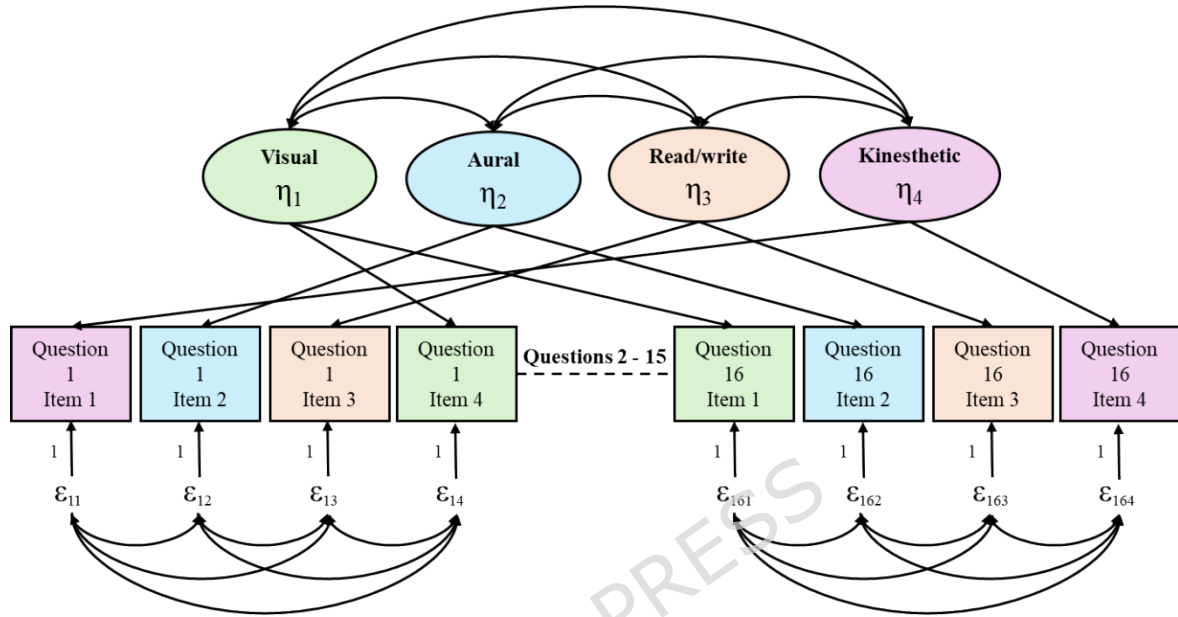
Figure 1. Correlated trait-correlated uniqueness model for VARK (CTCU)
