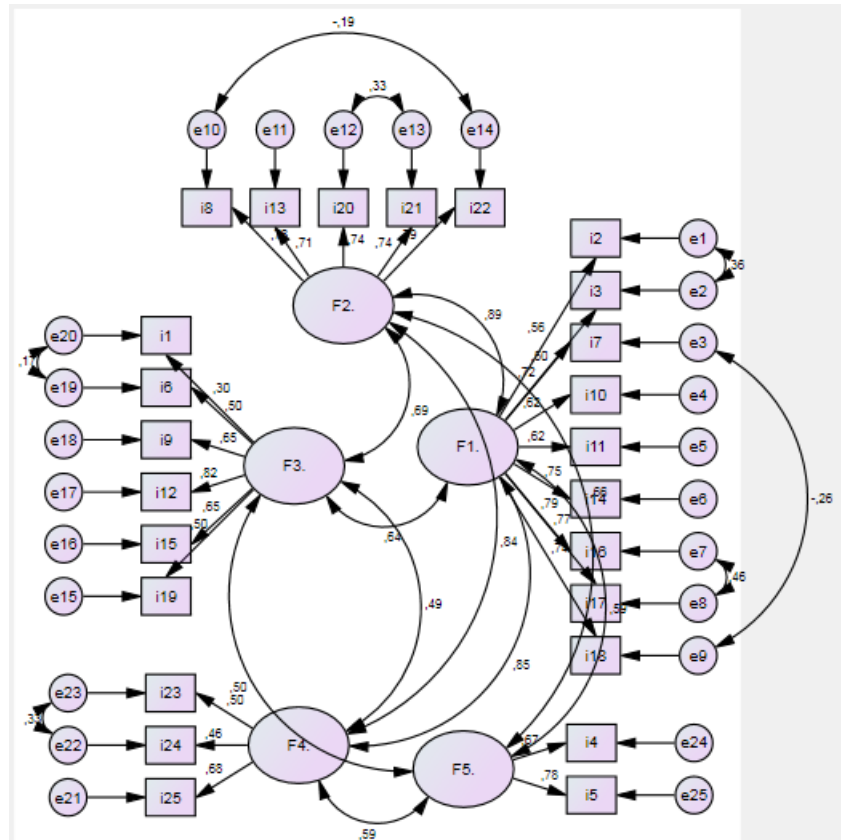
Figure 1. CFA results
