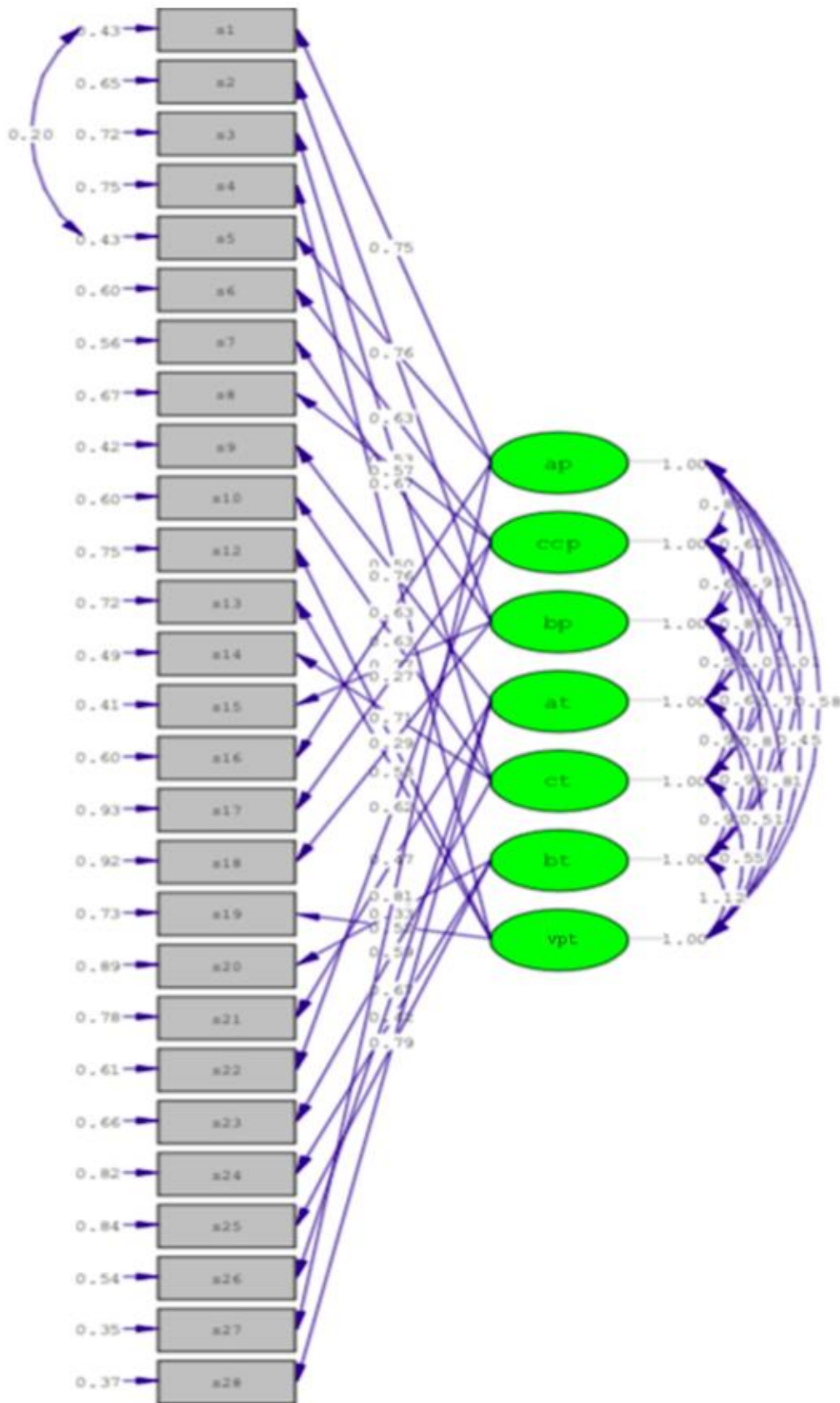
Figure 1. Confirmatory factor analysis model for the structure of model 2
