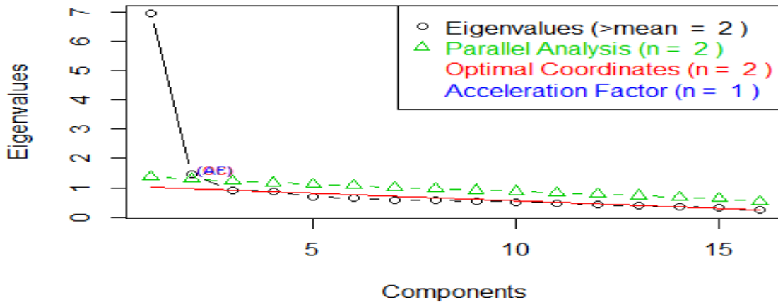
FIGURE 4. Eigenvalue-component graph
