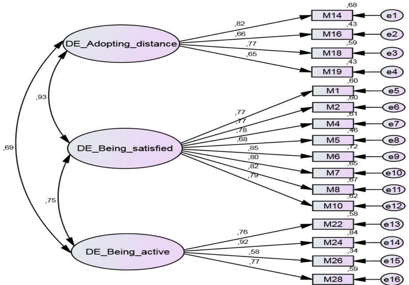
Figure 1. Confirmatory factor analysis scale structure
