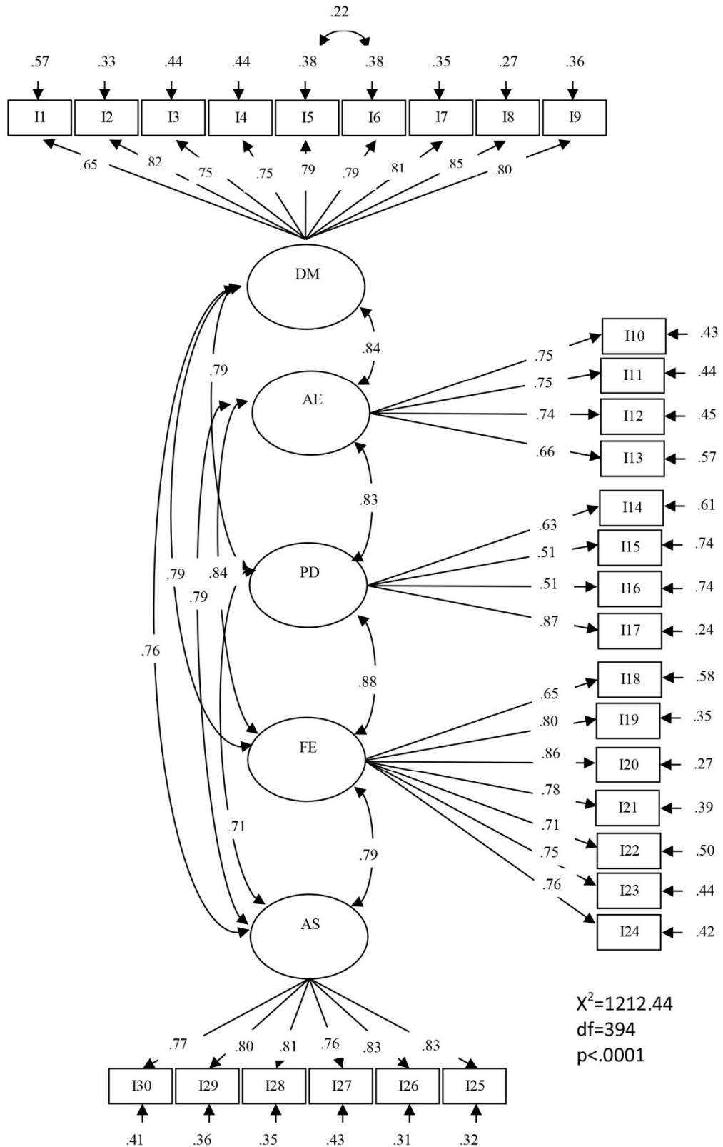
Figure 1. Path Diagram of TSES
