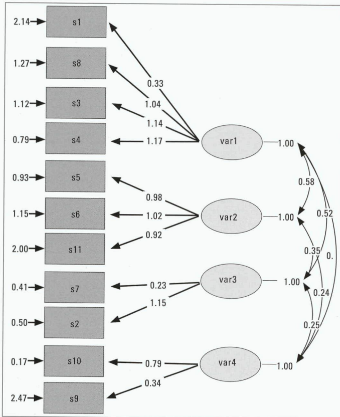
Figure 1. SEM for the EHfScB (Turkish Version) (n=494)
