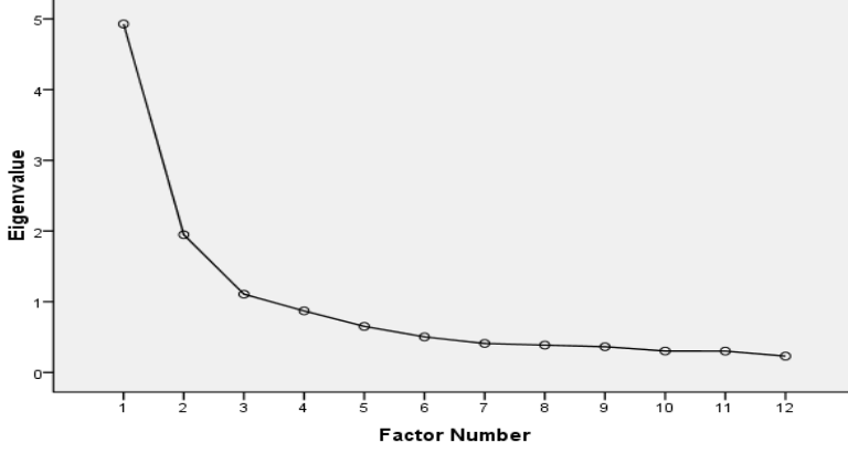
Scree Plot
